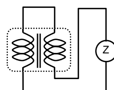
Differential Mode
